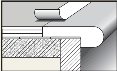
Standard Stair Nose
