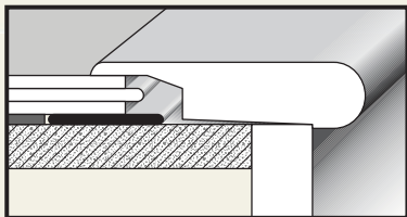
Overlap Stair Nose
